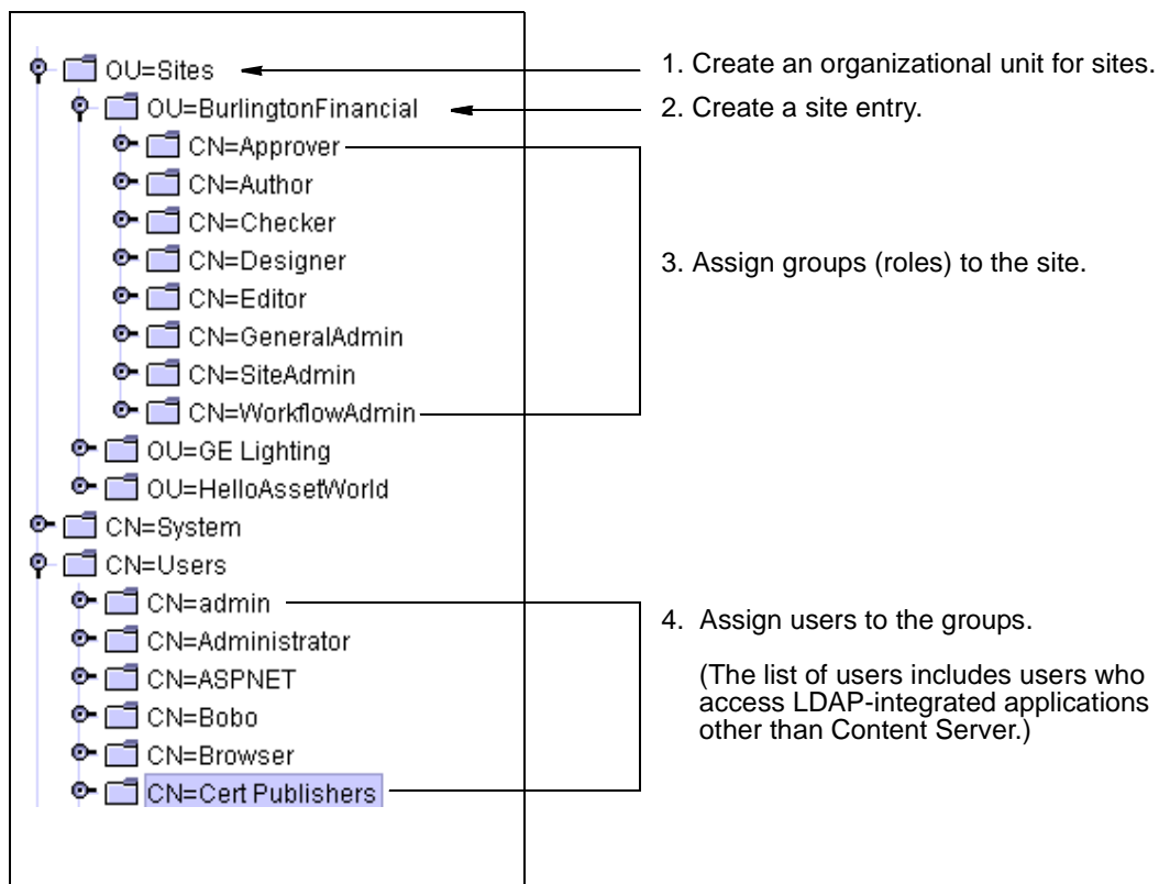
Figure 1: LDAP Hierarchies
